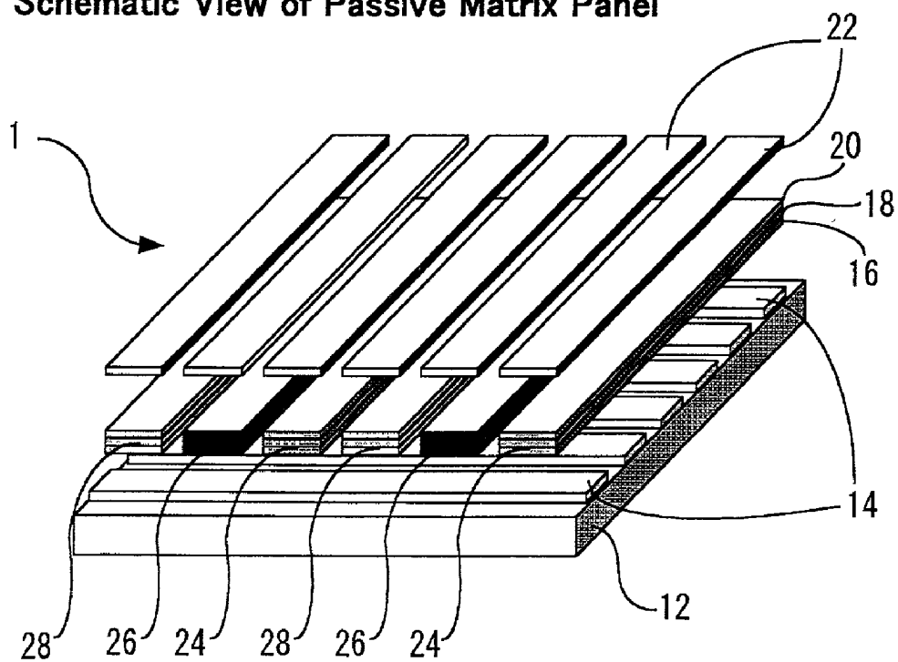
Schematic View of Passive Matrix Panel
